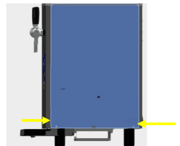
8. Secure the side panel with screws and fit lid securely on top.
