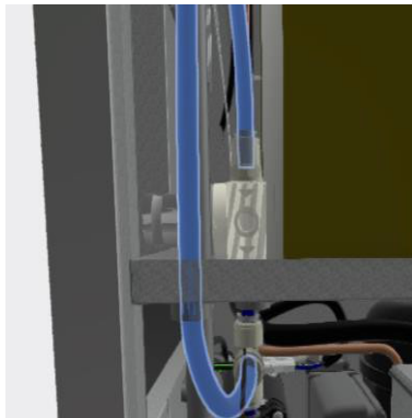
5. Remove both blue poly tubes from the regulator.
