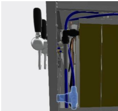
4. The regulator is behind the front plate with access from the side.
