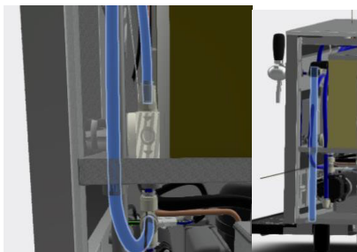
8. Connect both blue poly tubing to the regulator. Re-connect overflow tube.
